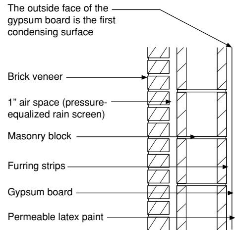
Figure 1: Potential for condensation in a masonry wall cavity in Tampa, Florida
