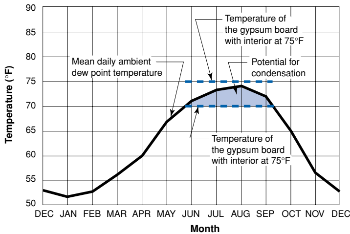
Figure 1: Potential for condensation in a masonry wall cavity in Tampa, Florida
