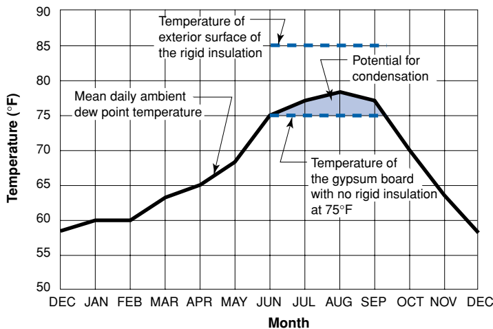
Figure 2: Potential for condensation in a masonry wall cavity in Miami, Florida
